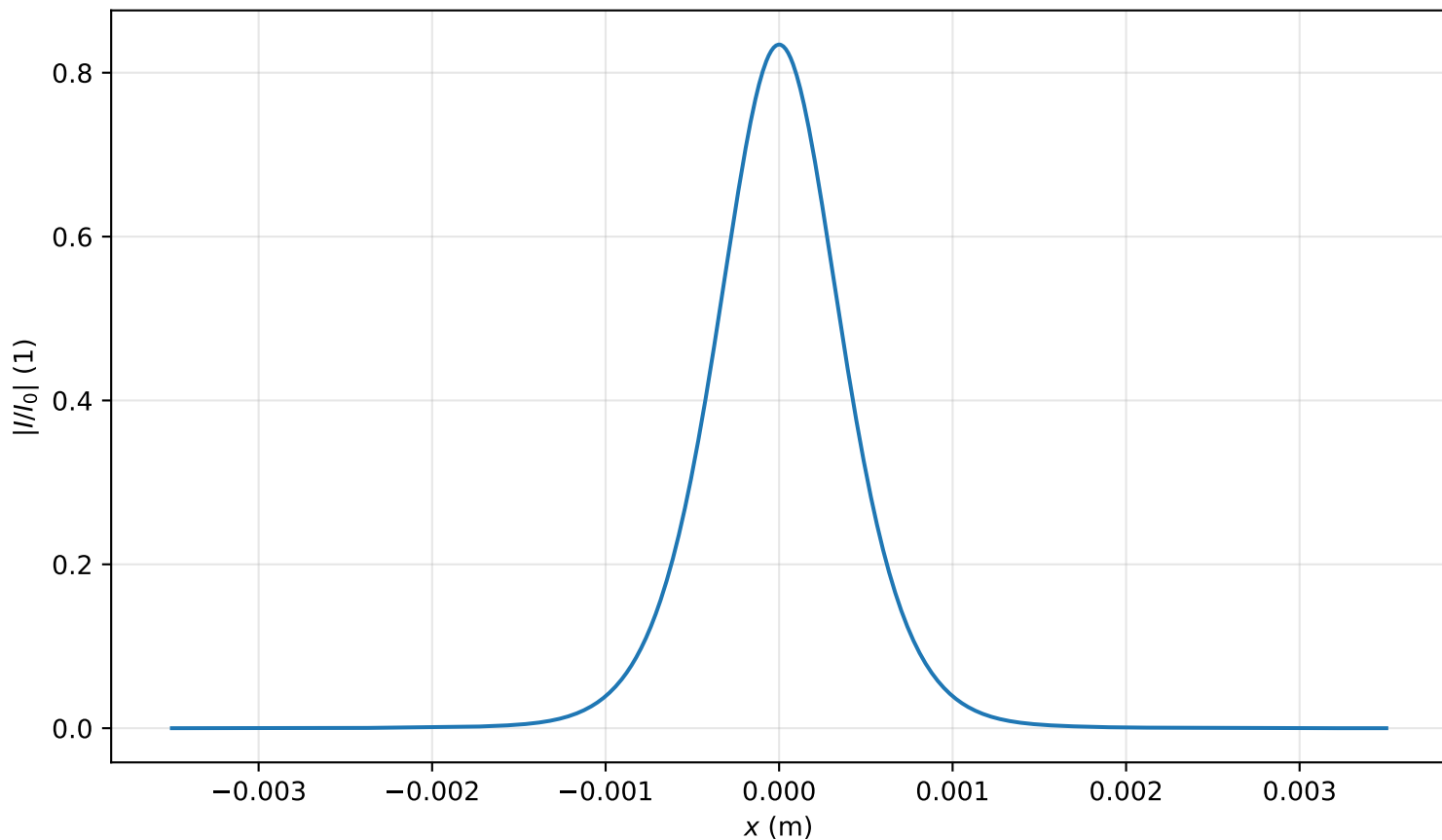
Intensity profile I(x, y = 0, z = 3.025m)/I_0 , P_{in}=0.7P_{cr} , artificial time
